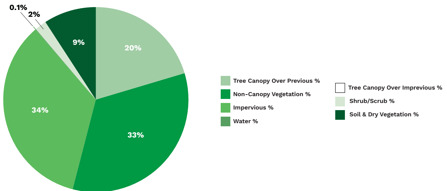
Figure 2. This illustrates the land cover composition of Uvalde based on imagery from 2022. TreePlotter CANOPY provides a more detailed assessment segmented by additional assessment.
