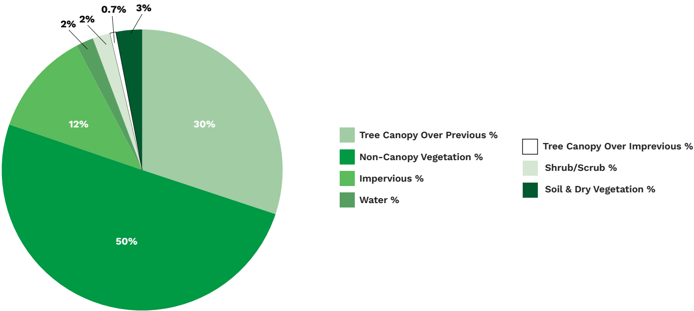
Figure 2. This illustrates the land cover composition of Seagoville based on imagery from 2022. TreePlotter CANOPY provides a more detailed assessment segmented by additional assessment.
