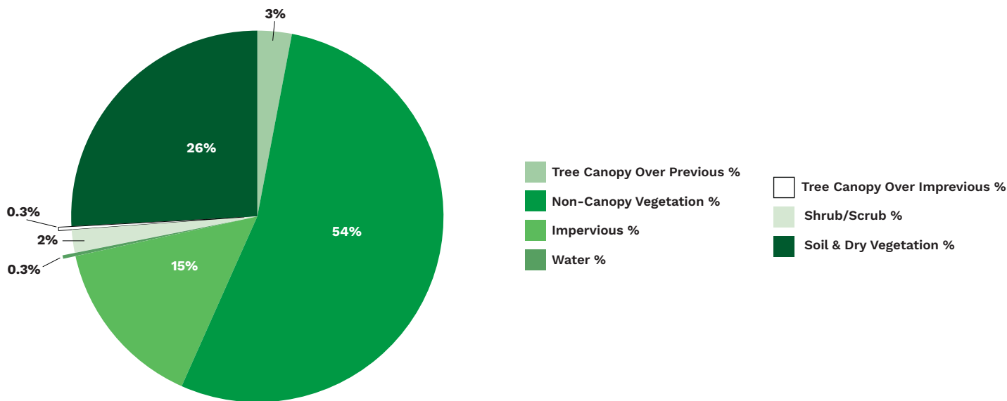
Figure 2. This illustrates the land cover composition of Robstown based on imagery from 2022. TreePlotter CANOPY provides a more detailed assessment segmented by additional assessment.
