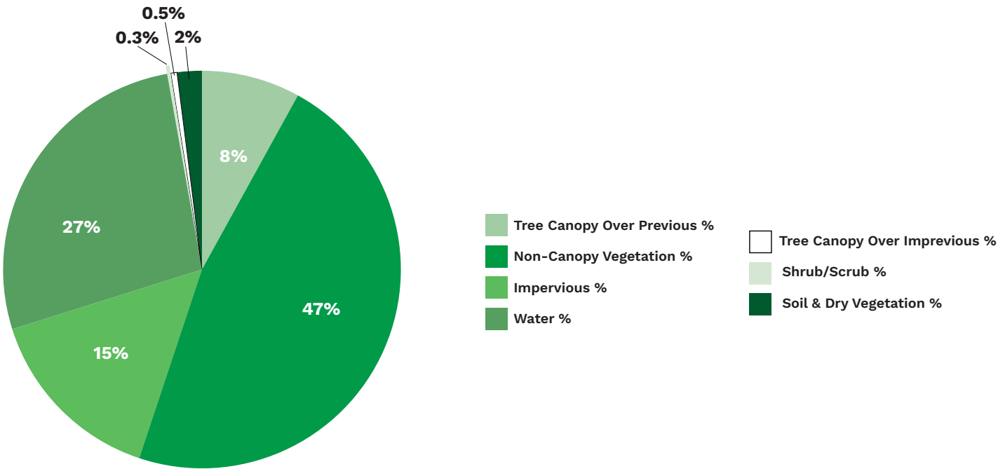
Figure 2. This illustrates the land cover composition of Port Lavaca based on imagery from 2022. TreePlotter CANOPY provides a more detailed assessment segmented by additional assessment.
