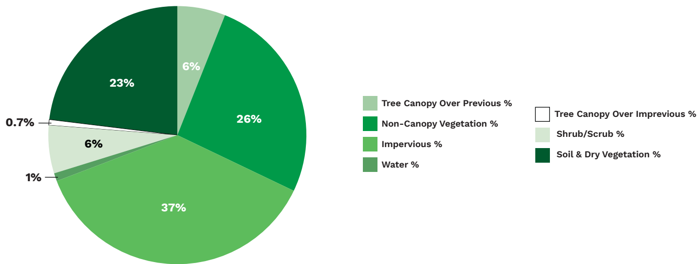
Figure 2. This illustrates the land cover composition of Eagle Pass based on imagery from 2022. TreePlotter CANOPY provides a more detailed assessment segmented by additional assessment.
