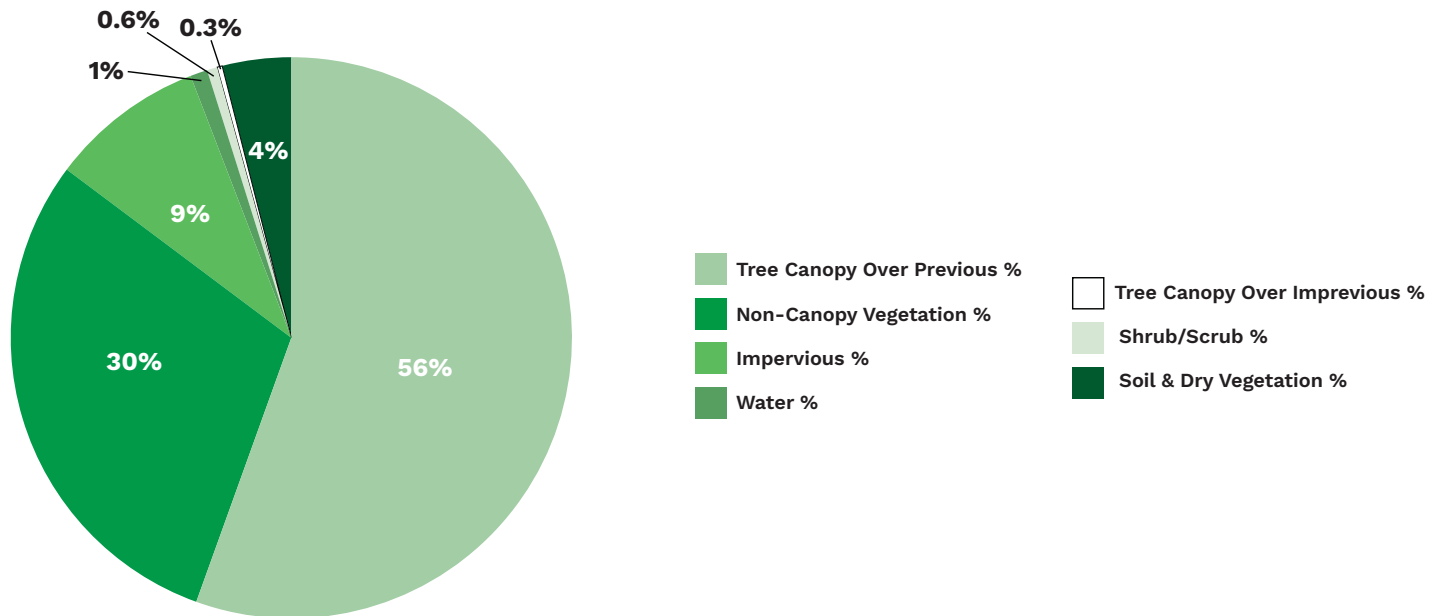
Figure 2. This illustrates the land cover composition of Cleveland based on imagery from 2022. TreePlotter CANOPY provides a more detailed assessment segmented by additional assessment.
