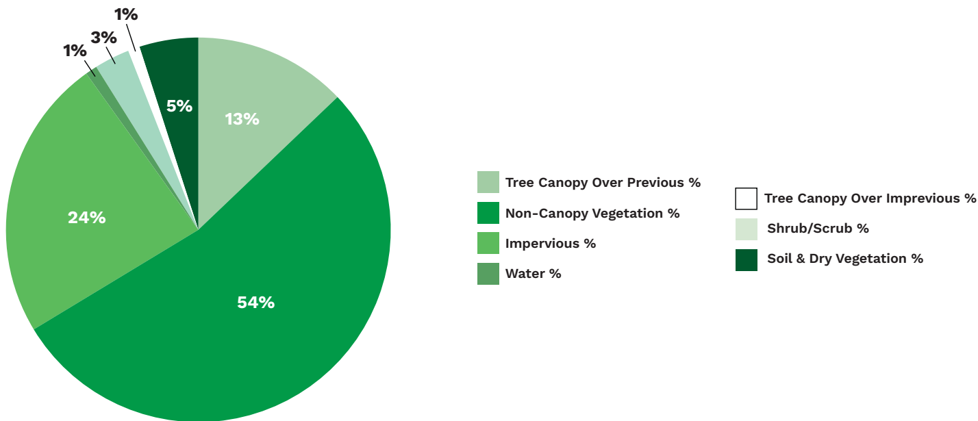
Figure 2. This illustrates the land cover composition of Alton based on imagery from 2022. TreePlotter CANOPY provides a more detailed assessment segmented by additional assessment.
