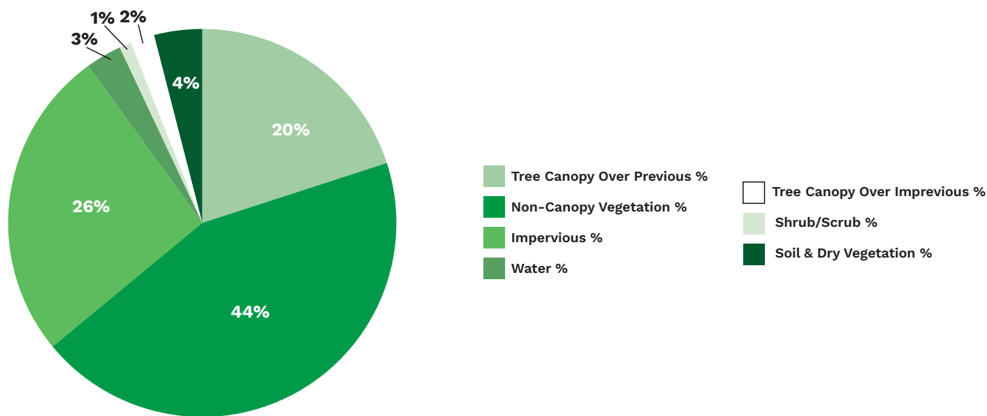
Figure 2. This illustrates the land cover composition of Alice based on imagery from 2022. TreePlotter CANOPY provides a more detailed assessment segmented by additional assessment.
