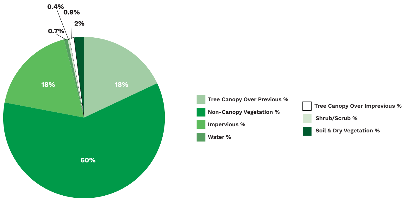
Figure 2. This illustrates the land cover composition of Navasota based on imagery from 2022. TreePlotter CANOPY provides a more detailed assessment segmented by additional assessment.
