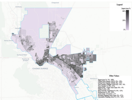
Stormwater runoff
