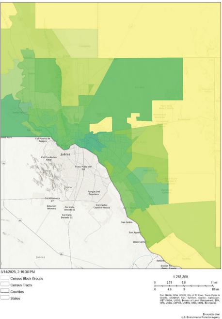
Air Quality
