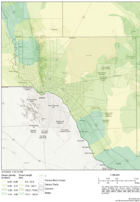
Water quality
